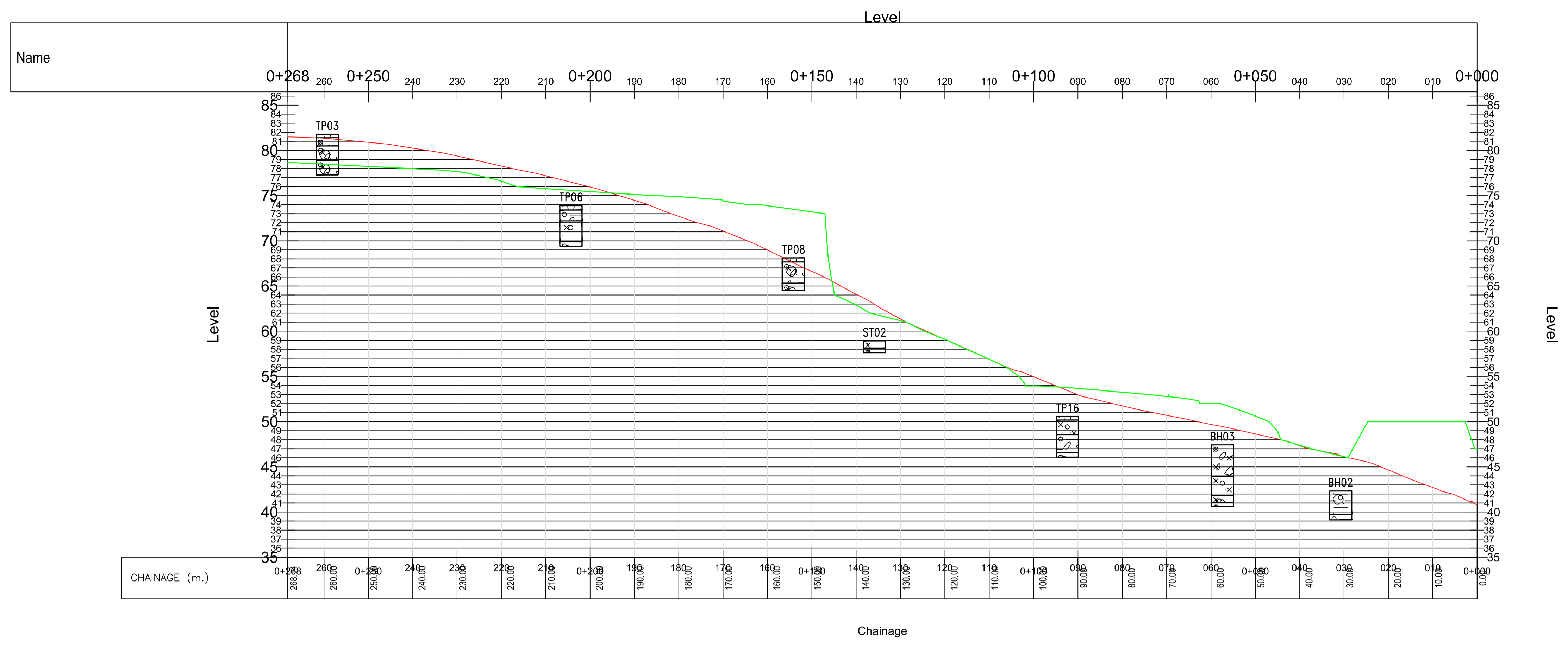
LONGSECTION OF BASELINE 4 - LONGSECTION 4 SCALE: H 1:500, V 1:245. DATUM: 35.000
